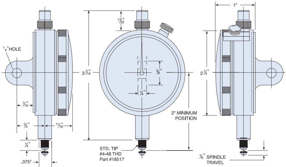
Indicator back options for High Amplification Group 2
