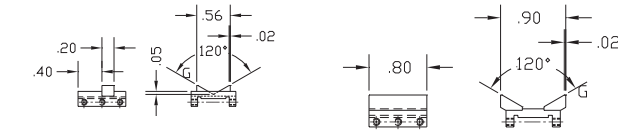
Work support No.5 Part #48572 .500" - 1.000" balls
