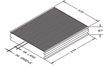
Part# 47402 Thin serration and flat reversible anvil
