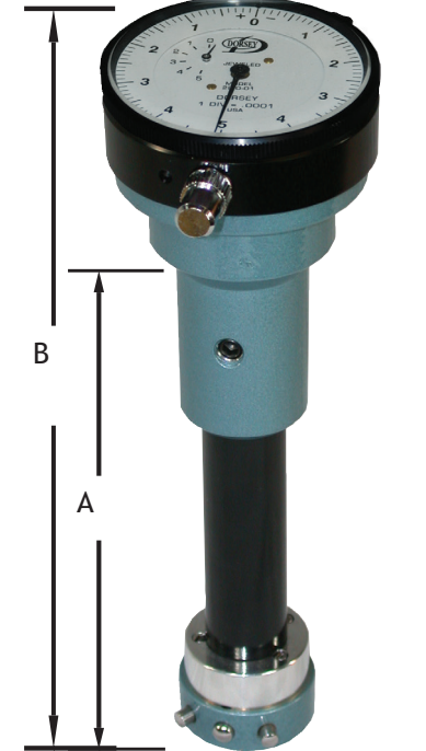
Perpendicular, Style 4 For vertical axis bores below eye level.
