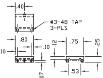
Work support blank Part #48582
