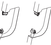
2 Wire or 3 wire floating carbide rolls on fixed carriers (plus special master) Best suited for heavy production inspection of pitch diameter on threads, screw forms, helical gears, and splines
