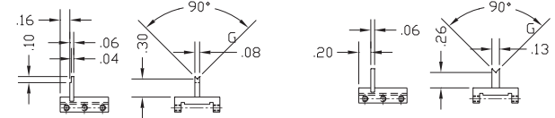
Work support No.1 Part #48568 .060" - .100" balls
