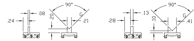
Work support No.3 Part #48570 .160" - .250" balls
